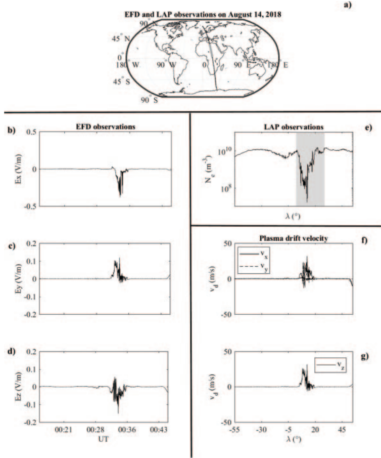
Fig. 1. – EFD and LAP observations by CSES-01 satellite on August 14, 2018. Panel (a) shows the location of the investigated orbit (solid black line) between 00:17 and 00:46 UT. The thick grey part underlines the time interval in which the EPB was detected by CSES-01. Panels (b), (c) and (d) display the electric field components. Panel (e) shows the electron density profile measured by the LAP. Panels (f) and (g) show the horizontal and the vertical plasma drift velocities. All components were expressed in the geographical reference frame. The grey shaded region represents the identification of the PB.
