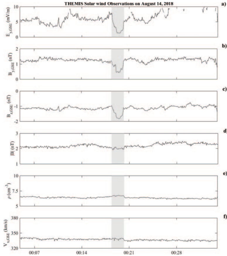
Fig. 2. – THEMIS-C solar wind observations: (a) Y_{GSE} component of the interplanetary electric field; (b) Y_{GSE} component of the interplanetary magnetic field; (c) Z_{GSE} component of the magnetic field; (d) total interplanetary magnetic field; (e) plasma density; (f) X_{GSE} component of the plasma velocity. All components were expressed in the geocentric-solar-ecliptic (GSE) reference frame.
