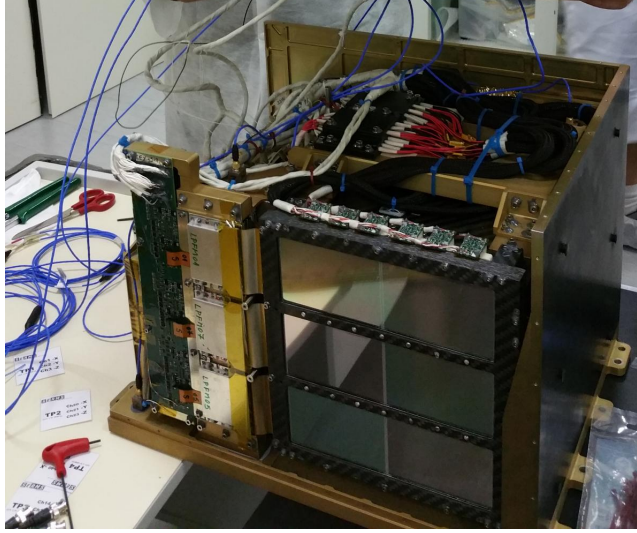
Figure 1.11: HEPD-01 detector. The tracker is visible in front of the setup [15].
