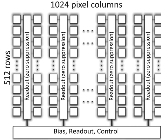
(a) Double column structure.
