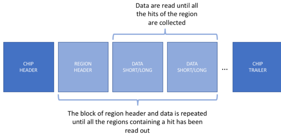
Figure 2.11: Readout logic of ALPIDE.
