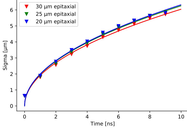
Figure 4.39: Evolution of \sigma of the electron density distribution over time during the first 10 ns after charge generation.
