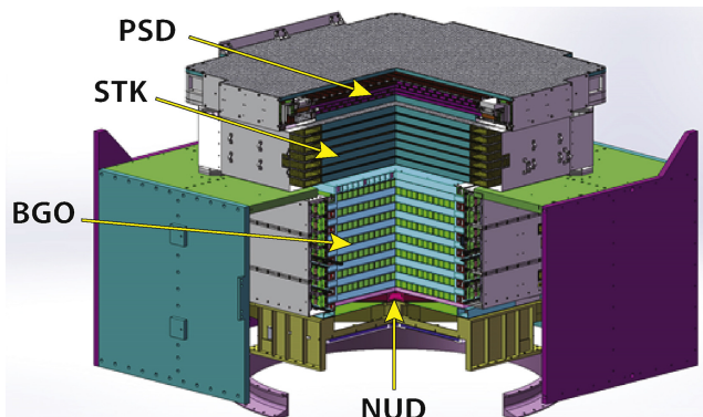
Figure 1.4: Dampe experiment [23].
