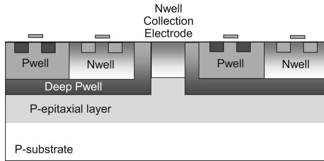
(c) Readout inside a deep p-well.
