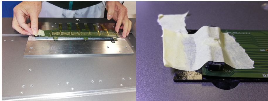
(a) Operations to glue the carbon fibre to the jig.
