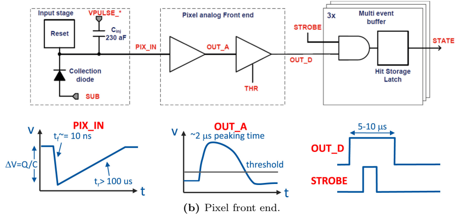
Figure 2.7: Details of structure of ALPIDE [72].
